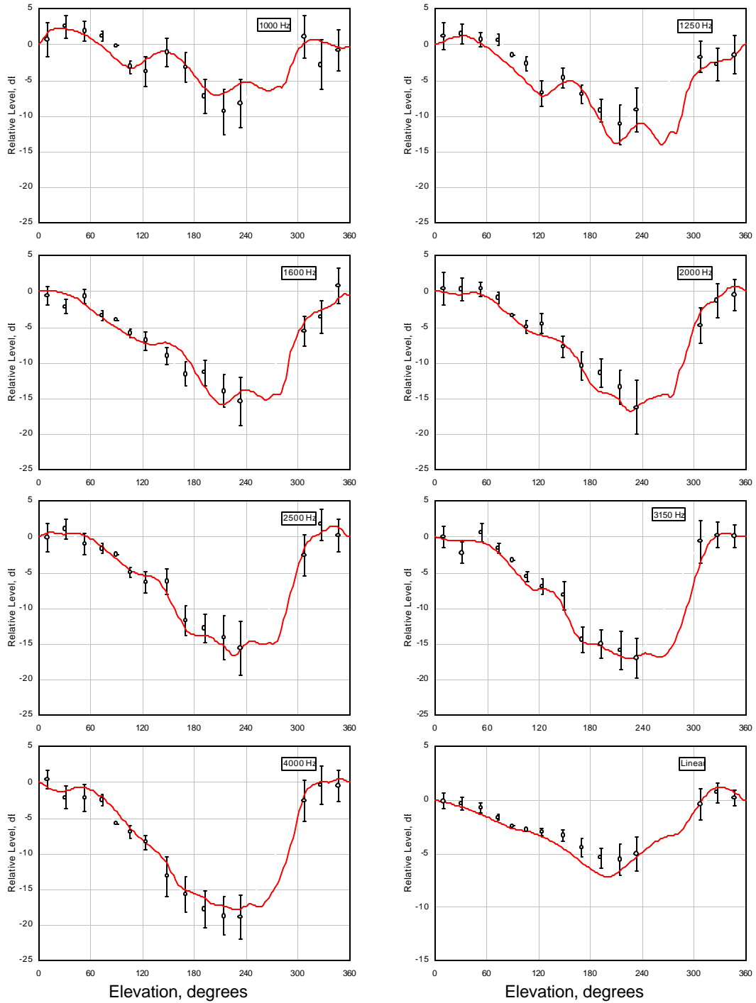
Figure 12 (cont.): Comparison of 1/3 octave band directivity results in the vertical plane between NRC (o) and Moreno & Pfromtznher (—). Vertical bars on NRC results represent \pm 1 standard deviation.
