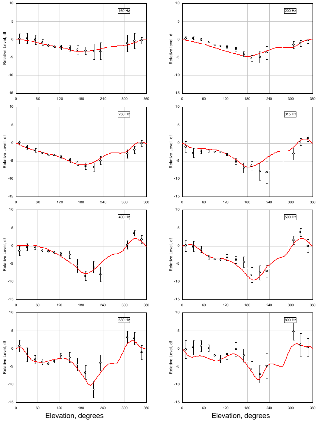
Figure 13: Comparison of 1/3 octave band directivity results in the vertical plane between NRC (o) and Moreno & Pfretzschner (—). Vertical bars on NRC results represent \pm 1 standard deviation.
