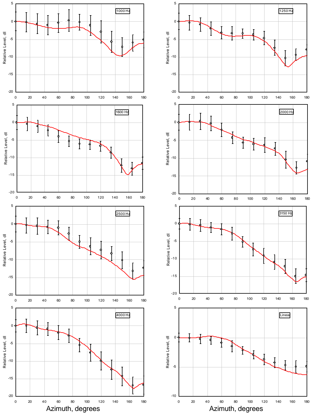
Figure 11 (cont.): Comparison of 1/3-octave band directivity results in the horizontal plane between NRC (o) and Moreno & Pfretzschner (—). Vertical bars on NRC results represent \pm 1 standard deviation.
