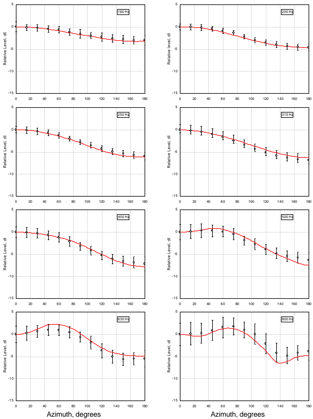
Figure 12: Comparison of 1/3 octave band directivity results in the horizontal plane between NRC (o) and Moreno & Pfretzschner (—). Vertical bars on NRC results represent \pm 1 standard deviation.
