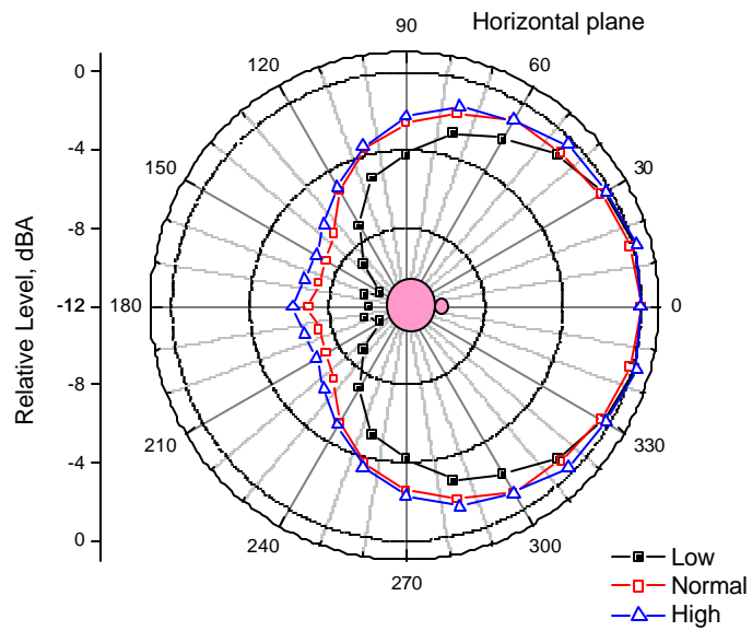
Figure 5: Directivity patterns of the relative A-weighted levels of a male talker speaking at three different voice levels.
