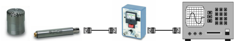
Fig 7. Prepolarized set-up
