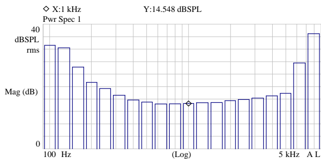
Fig 5. Typical Noise Floor Data, 1/3 Octave Band Analysis
